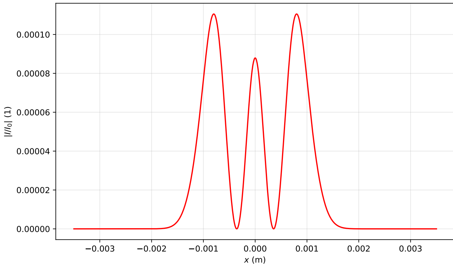
Intensity profile I(x, y = 0, z = 0.398)/I_0 , P_{in}=1.0P_{cr} , artificial time
